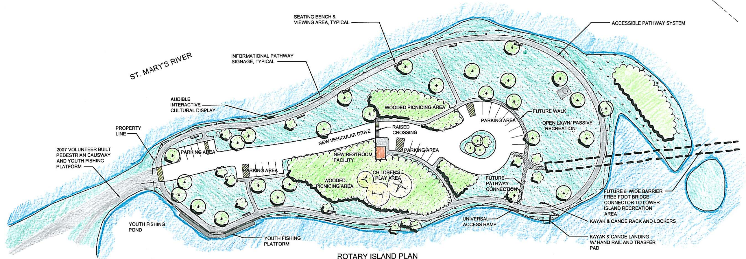
ROTARY ISLAND PLAN SCALE: 1" = 40'
