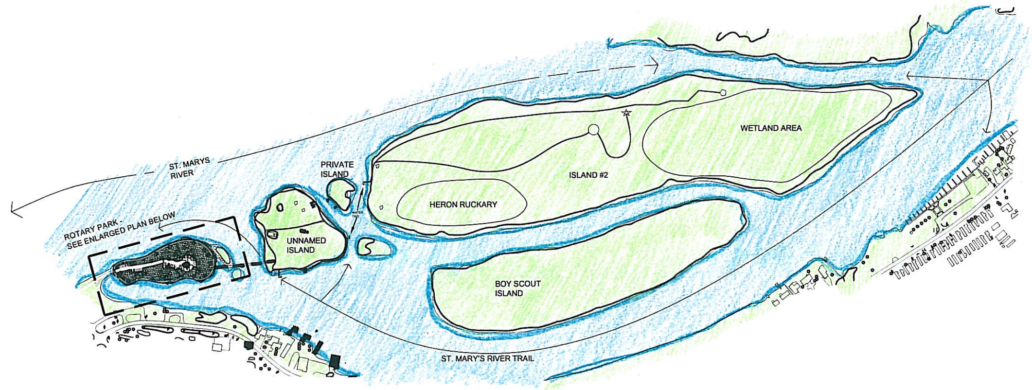
LOWER RIVER ISLANDS RECREATION PLAN SCALE: 1" = 300'
